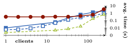
Fig. 3.10: Query 3 response time ( log-log plot )
