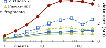
Fig. 3.2: Server network traffic
