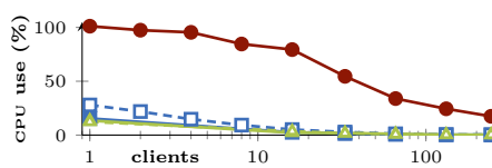
Fig. 3.7: Client processor usage per core
