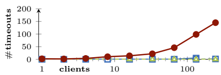
Fig. 3.3: Query timeouts
